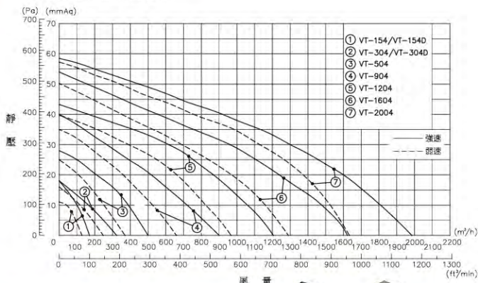
● 靜壓風量曲線表
